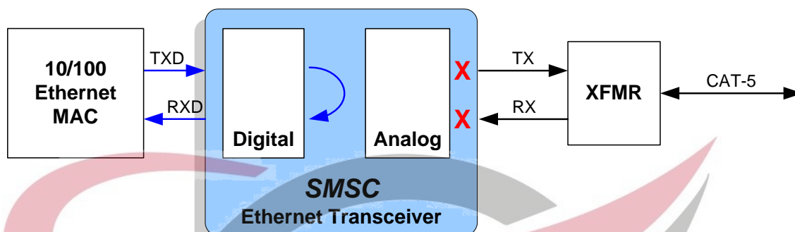
Figure 3.9 Near-end Loopback Block Diagram
